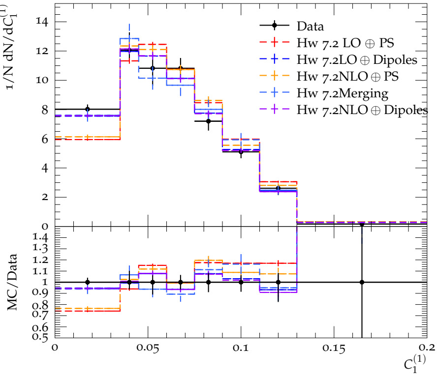
CMS, 13 TeV, t\bar{t} lepton+jets, gluon jets, charged particles
