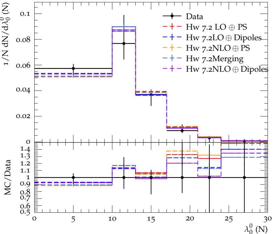
CMS, 13 TeV, t\bar{t} lepton+jets, light jets, all particles
