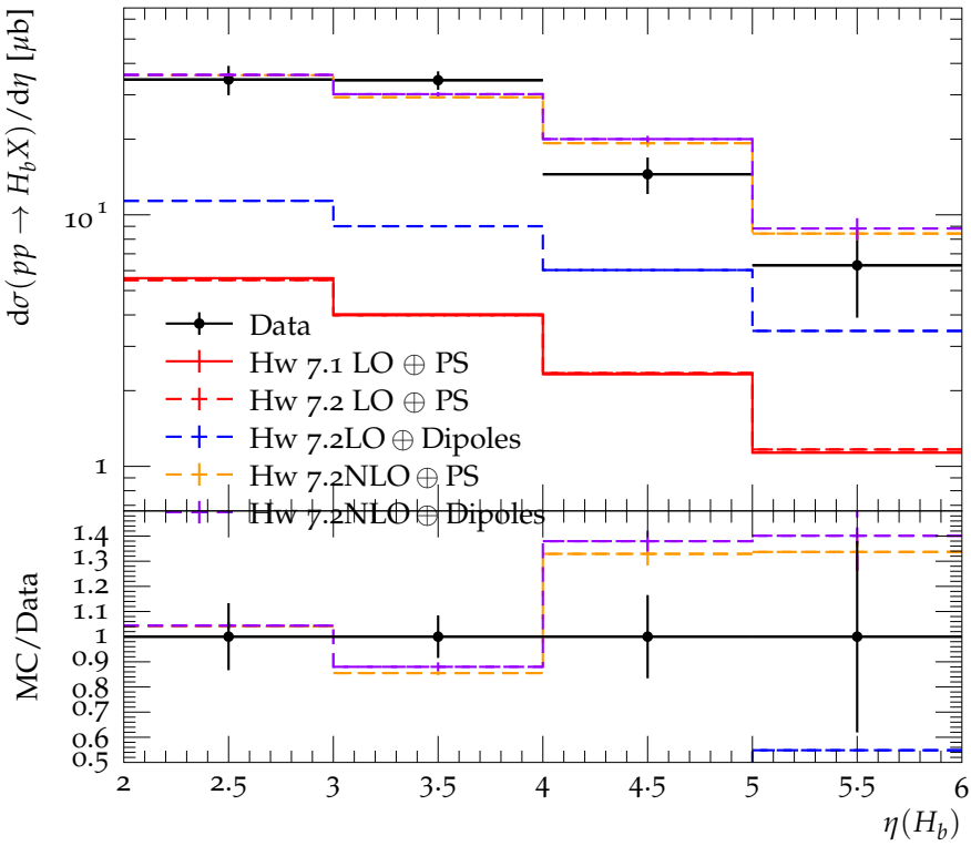
b production cross-section at \sqrt{s} = 7 TeV, with Tevatron fragmentation
