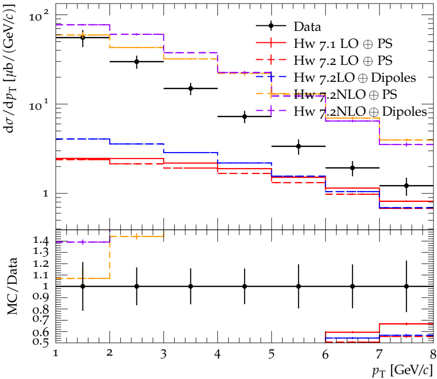
Prompt D^+ + c.c. d\sigma/dp_T for rapidity interval 2.0 < y < 2.5
