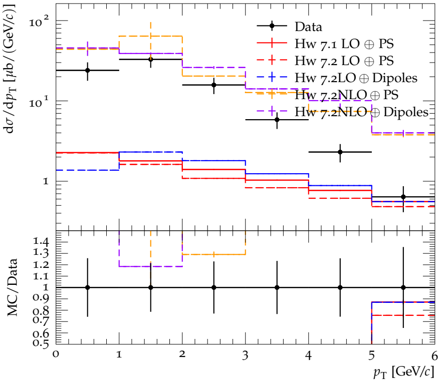
Prompt D^+ + c.c. d\sigma/dp_T for rapidity interval 4.0 < y < 4.5
