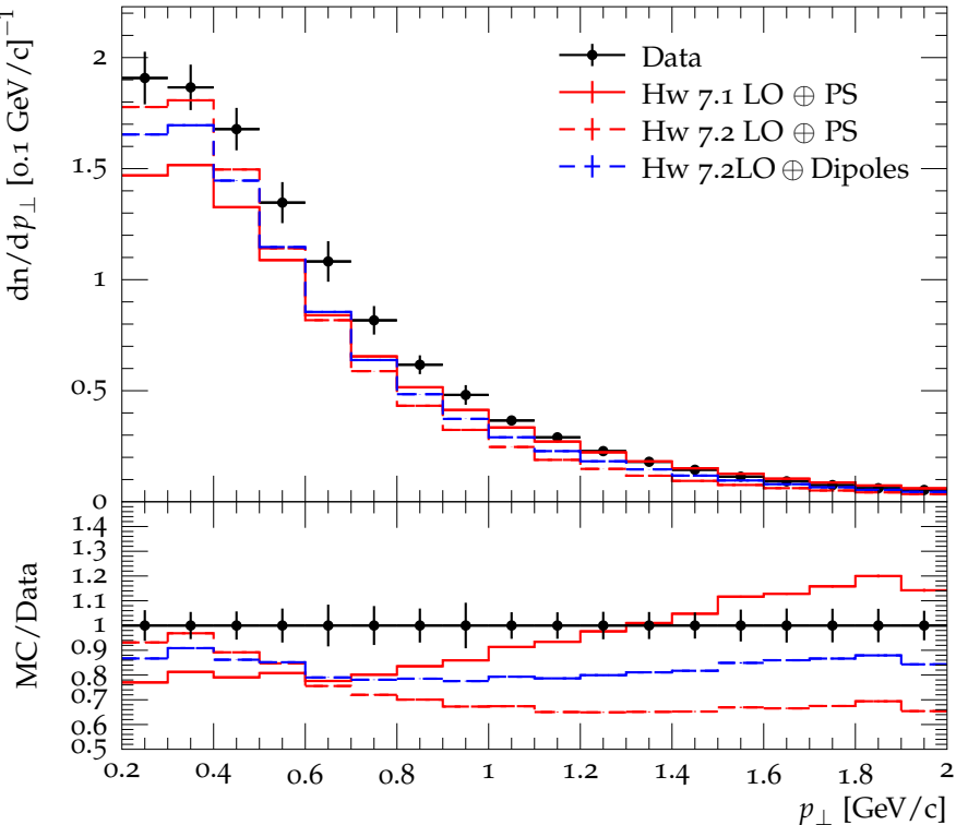
Prompt charged particle density at \sqrt{s} = 7 TeV
