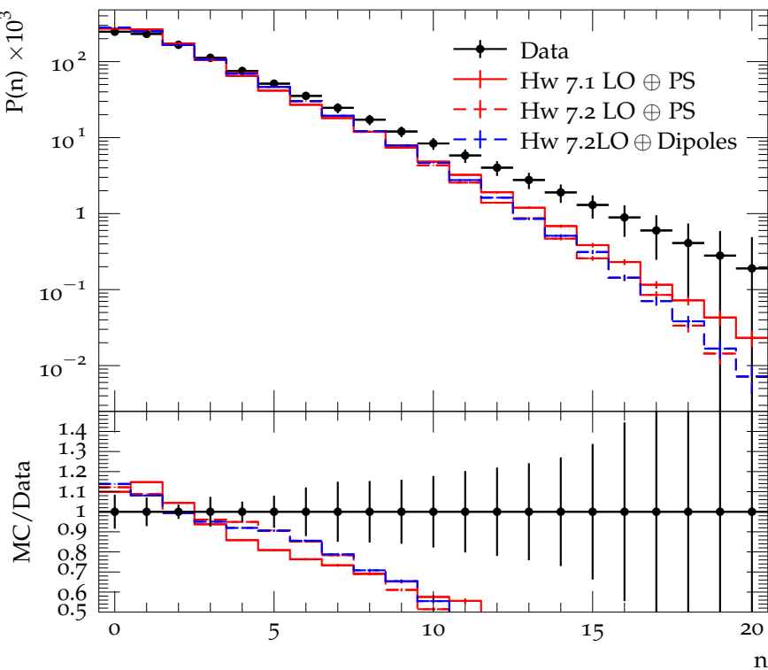
Ch. particle distribution at \sqrt{s} = 7 TeV ( 3.0 < \eta < 3.5 )
