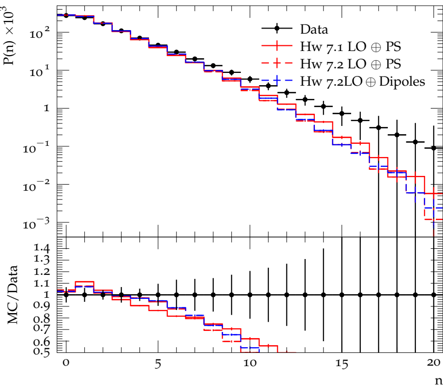
Ch. particle distribution at \sqrt{s} = 7 TeV ( 3.5 < \eta < 4.0 )
