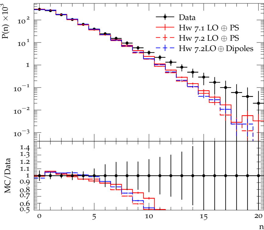
Ch. particle distribution at \sqrt{s} = 7 TeV ( 4.0 < \eta < 4.5 )
