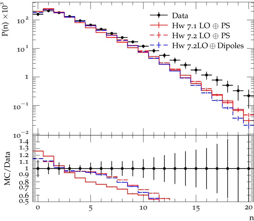
Ch. particle distribution at \sqrt{s} = 7 TeV ( 0.4 < p_{\perp} < 0.6 GeV/c)
