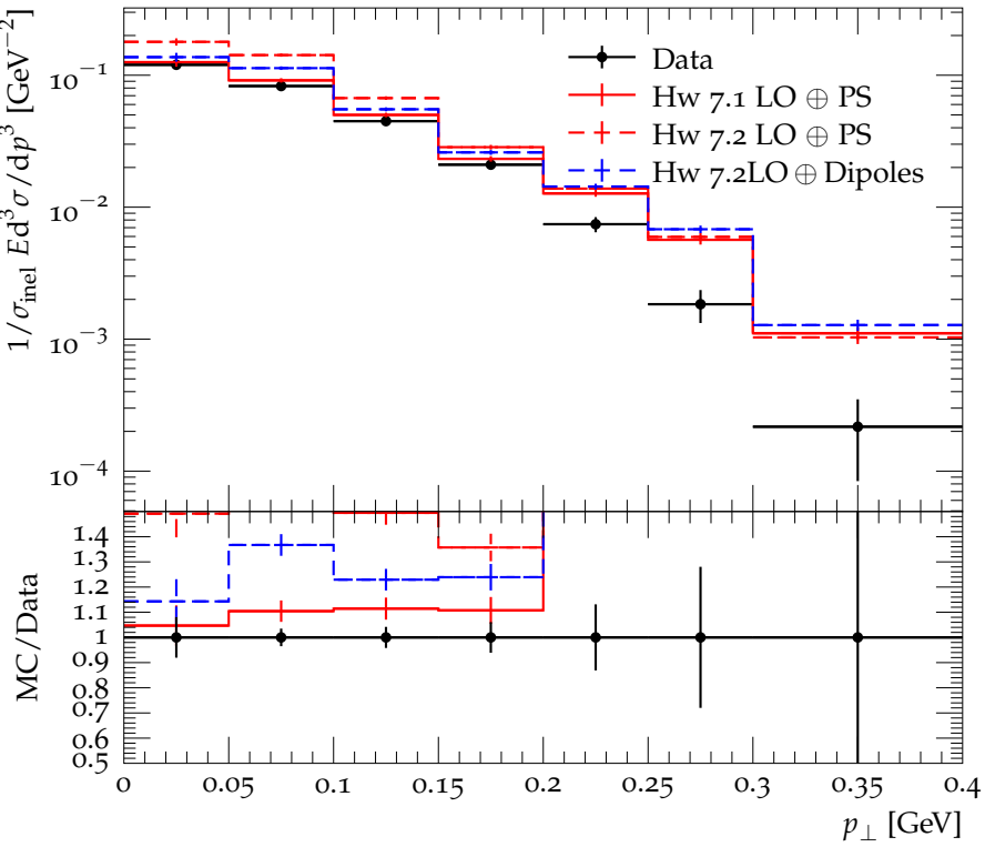
\pi^0 p_{\perp} spectrum, 9.6 < y < 10.0
