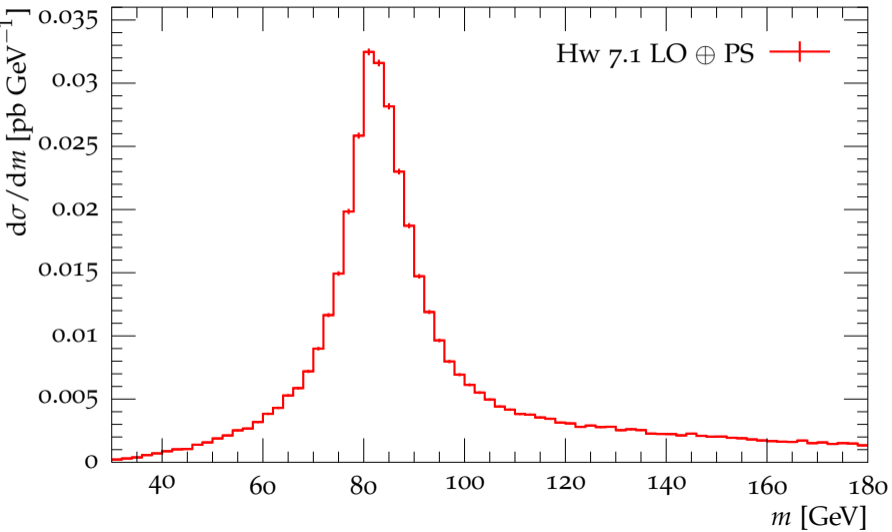
Mass distribution for W bosons
