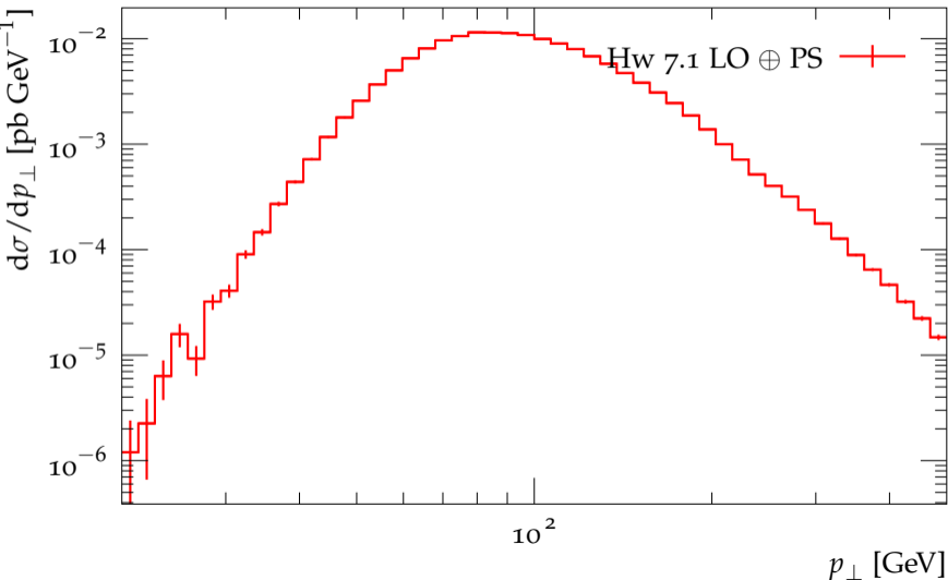
Transverse momentum distribution for jet 1
