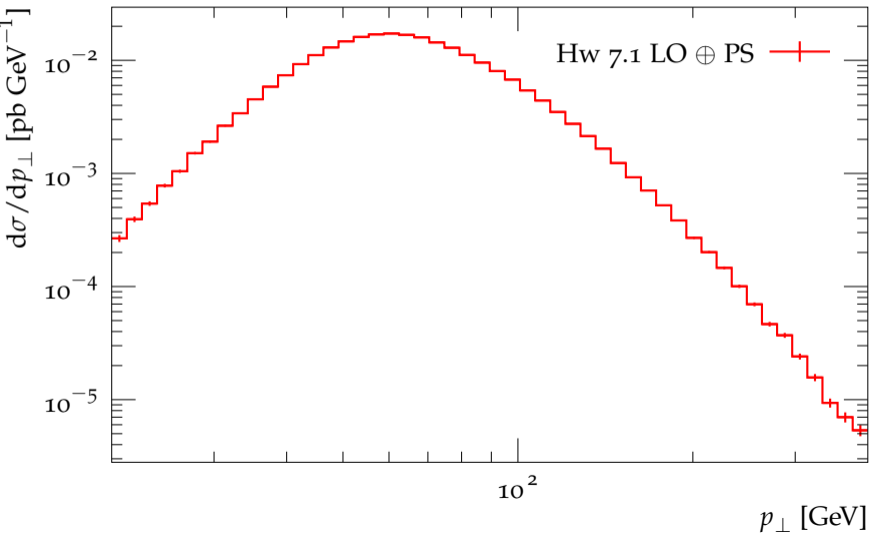
Transverse momentum distribution for jet 2
