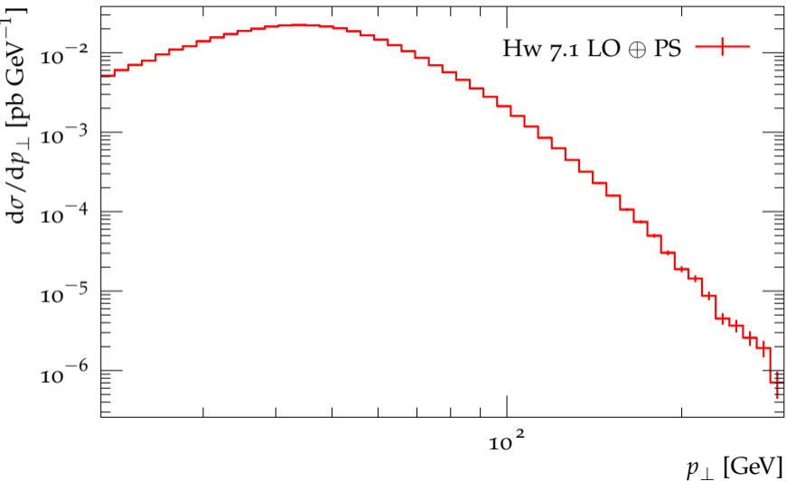
Transverse momentum distribution for jet 3
