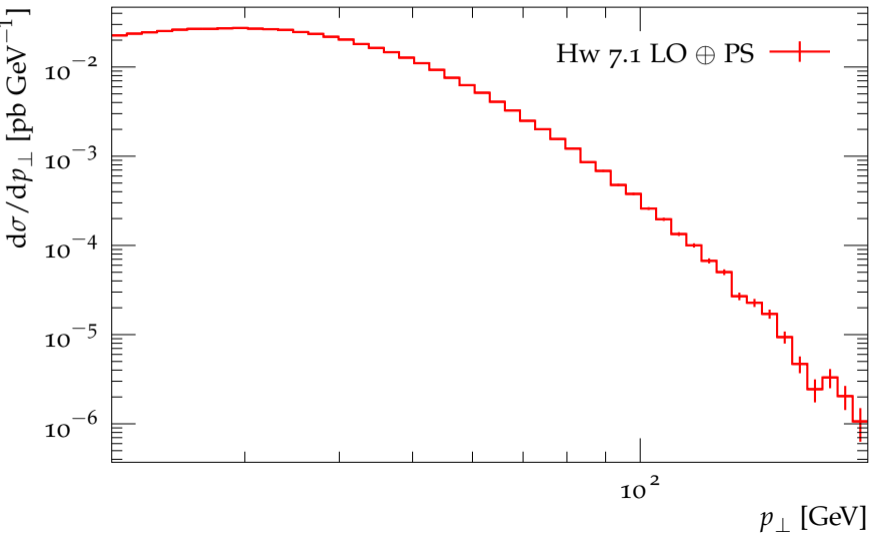
Transverse momentum distribution for jet 4
