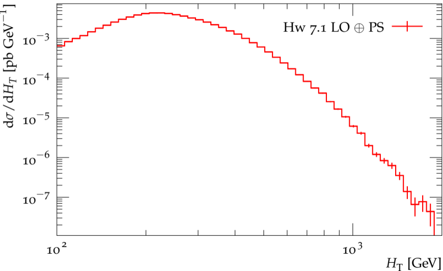
H_T distribution for all jets
