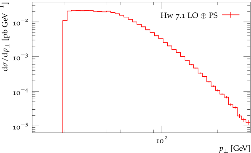
Transverse momentum distribution for b -jet 2
