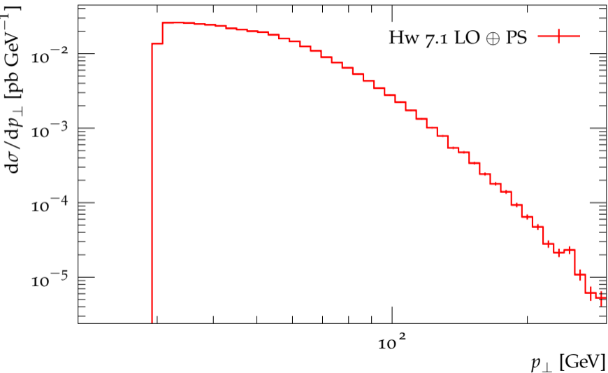
Transverse momentum distribution for light jet 2
