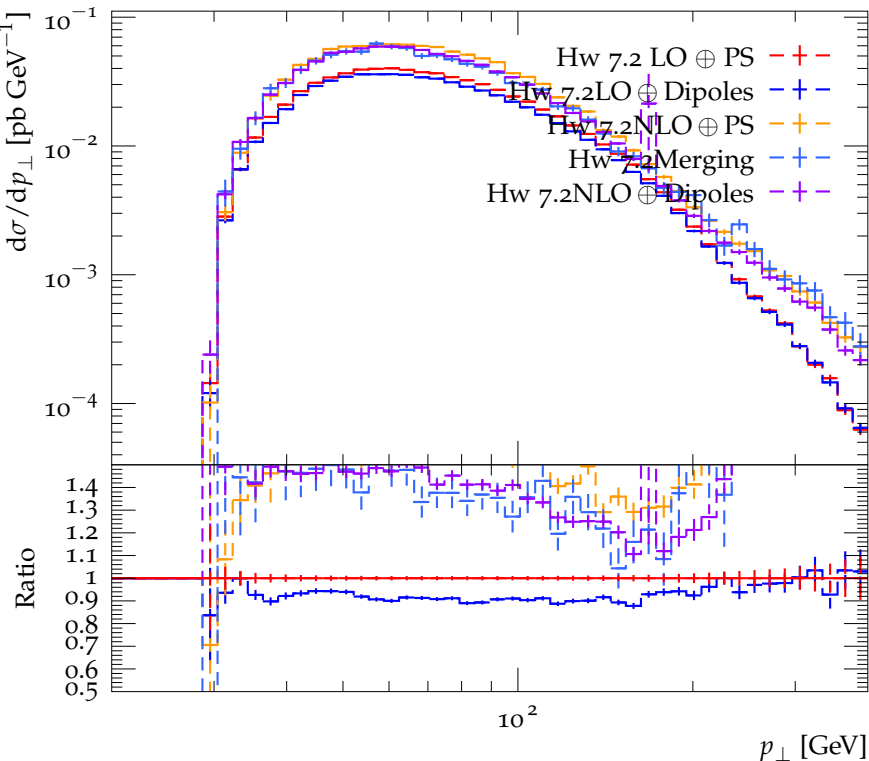
Transverse momentum distribution for light jet 1 ( N_\ell = 1 )
