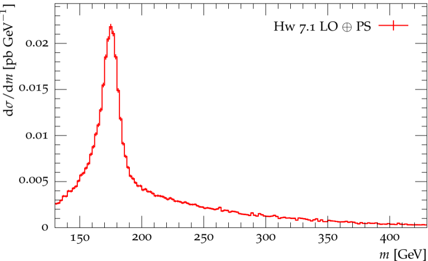
Mass distribution for reconstructed top after m_W cut
