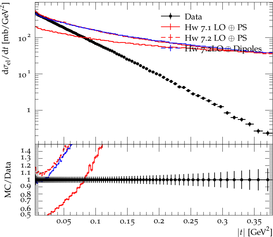
Differential elastic cross-section vs. |t| (low t )
