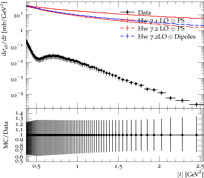
Differential elastic cross-section vs. |t| (high t )
