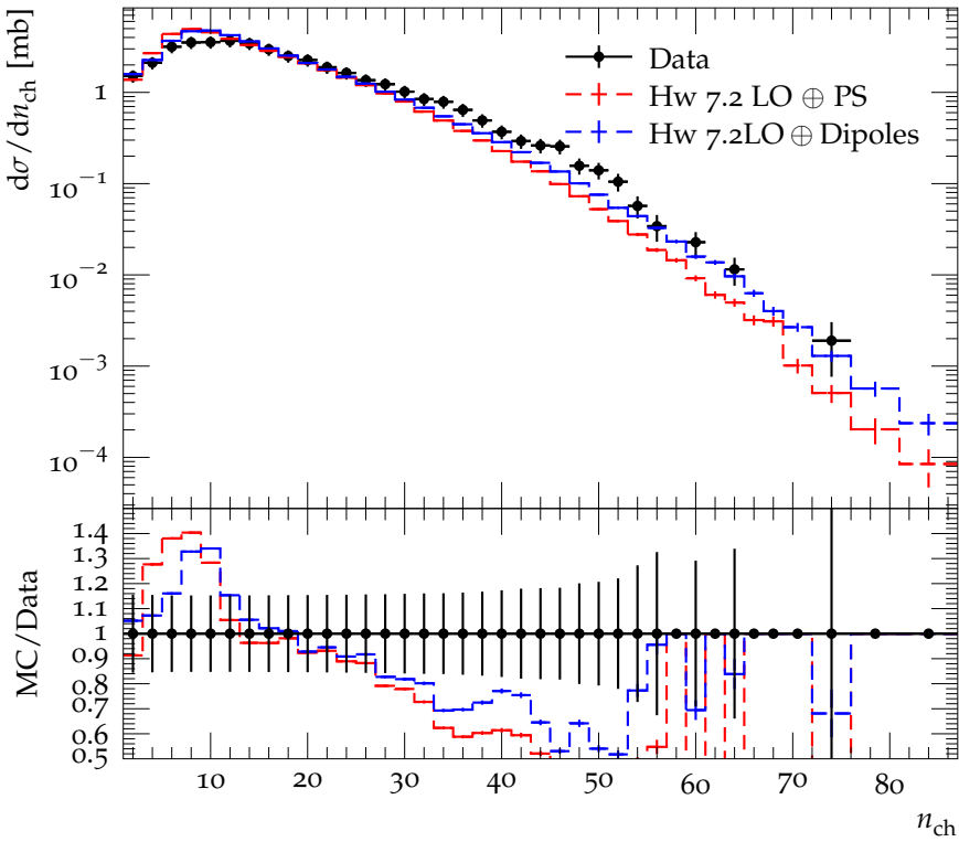
Multiplicity distribution at \sqrt{s} = 500 GeV
