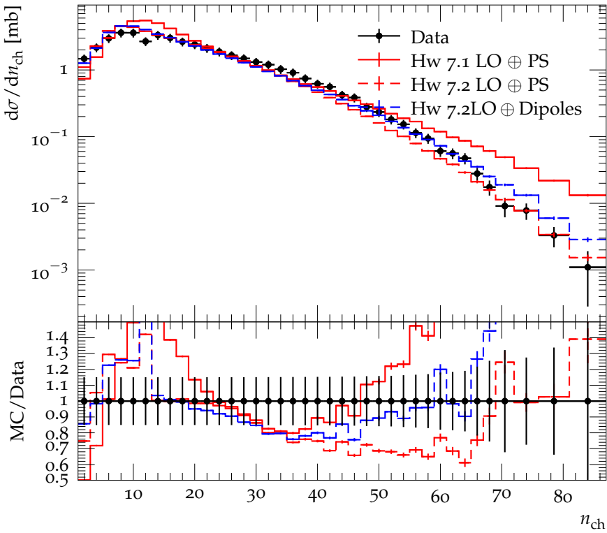
Multiplicity distribution at \sqrt{s} = 900 GeV
