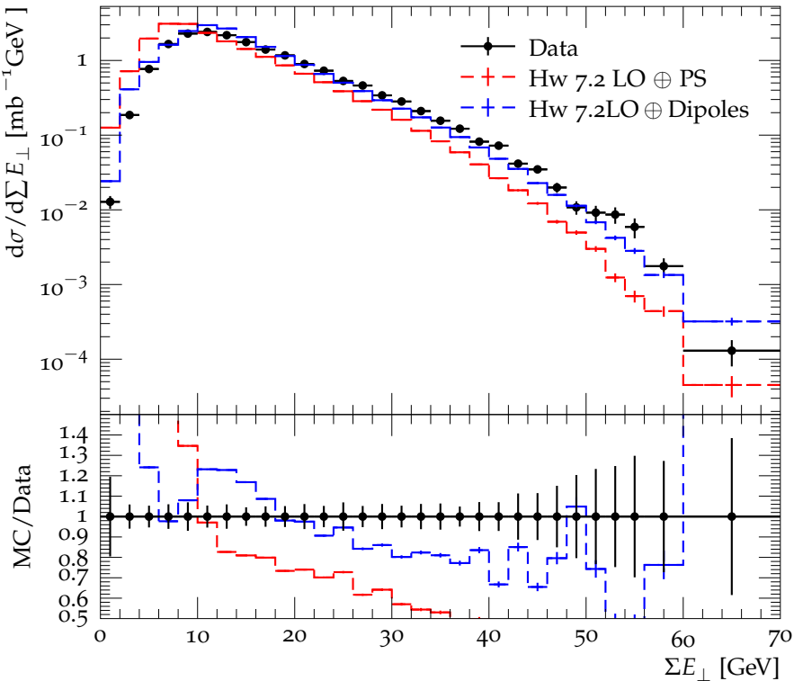
Transverse energy cross section at \sqrt{s} = 200 GeV and |\eta| < 6
