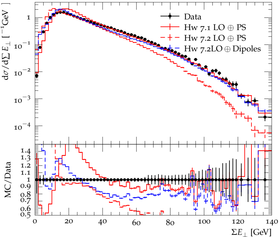
Transverse energy cross section at \sqrt{s} = 900 GeV and |\eta| < 6
