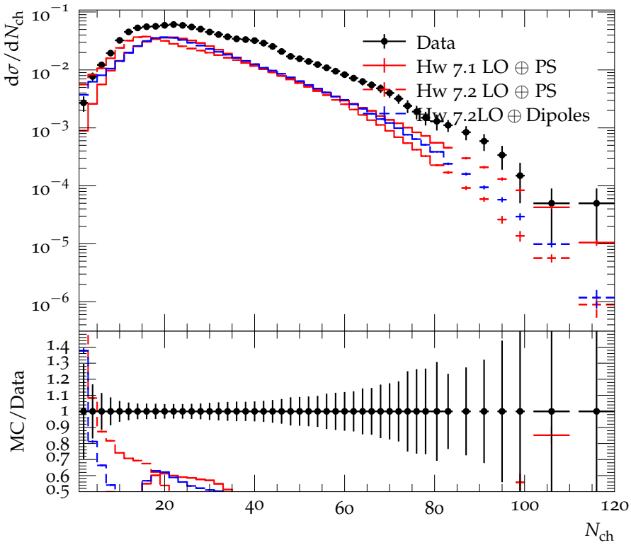
Charged multiplicity at \sqrt{s} = 546 GeV, |\eta| < 5.0
