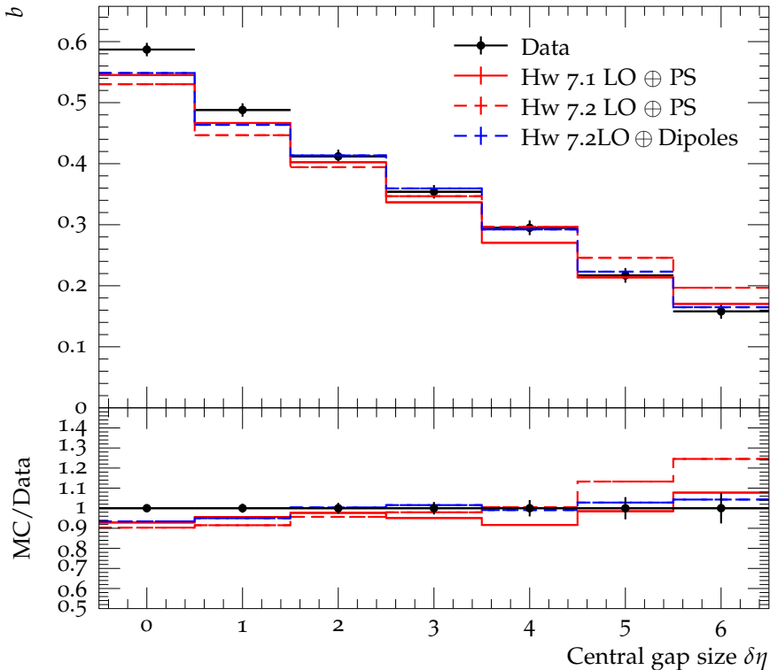
Forward-backward correlation b vs. gap size \sqrt{s} = 546
