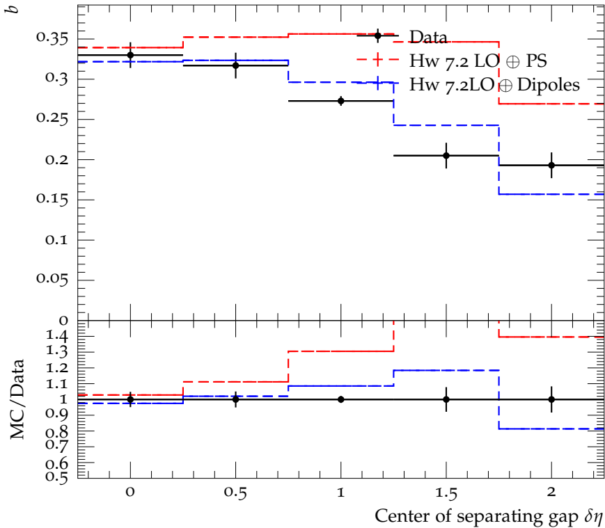
Forward-backward correlation b vs. gap center \sqrt{s} = 200
