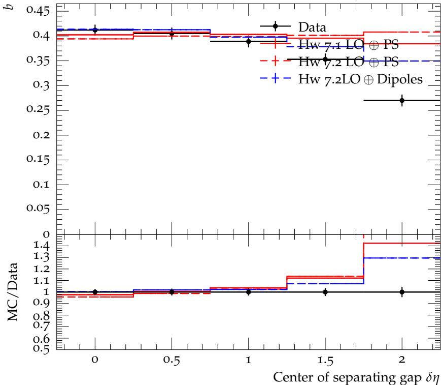
Forward-backward correlation b vs. gap center \sqrt{s} = 546
