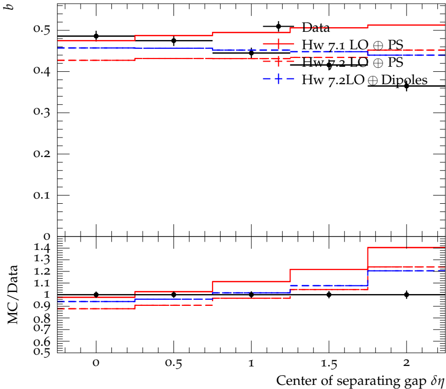
Forward-backward correlation b vs. gap center \sqrt{s} = 900
