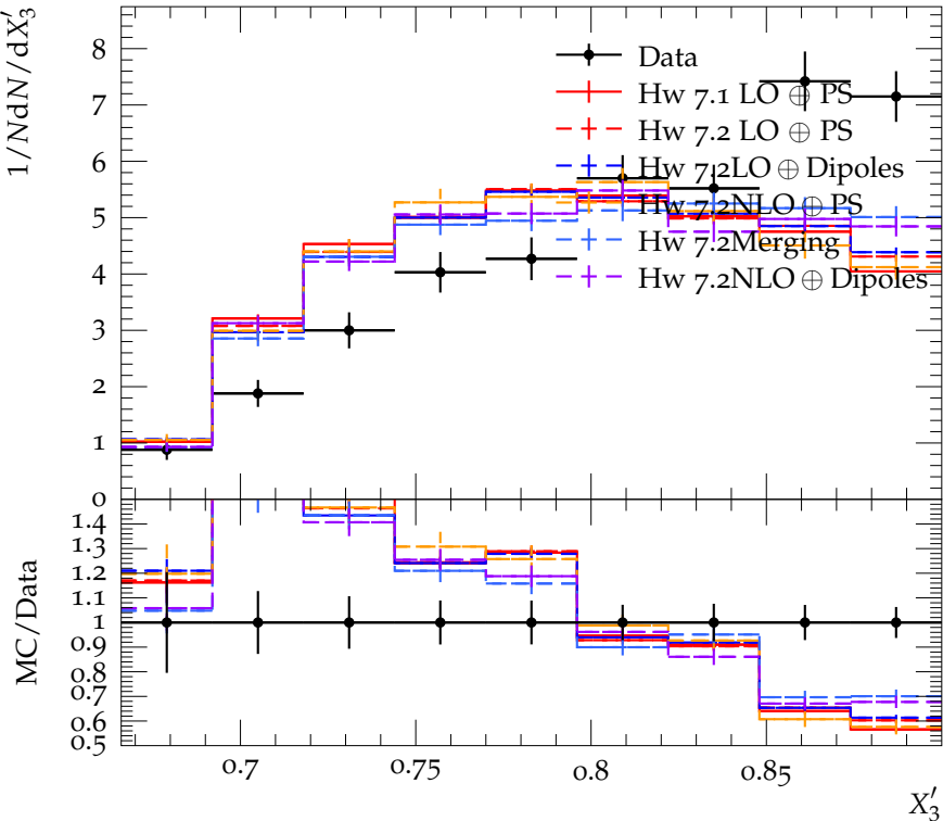
Dalitz distribution in inclusive 4-jet events
