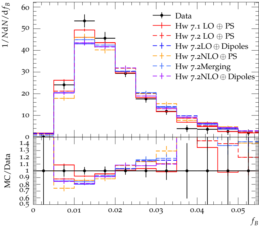
Single-body mass fraction in inclusive 4-jet events
