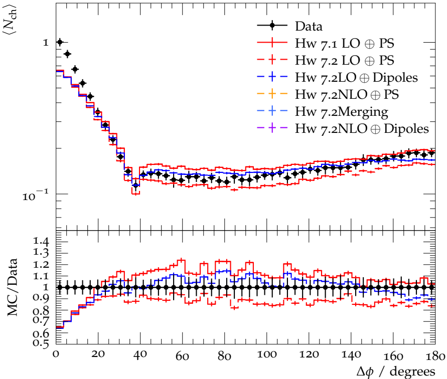
\langle N_{\text{ch}} \rangle vs. \Delta\phi from leading jet ( p_{\perp}^{\text{lead}} > 5 \text{ GeV} )
