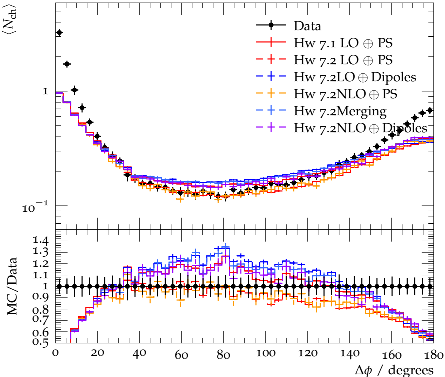
\langle N_{\text{ch}} \rangle vs. \Delta\phi from leading jet ( p_{\perp}^{\text{lead}} > 30 GeV)
