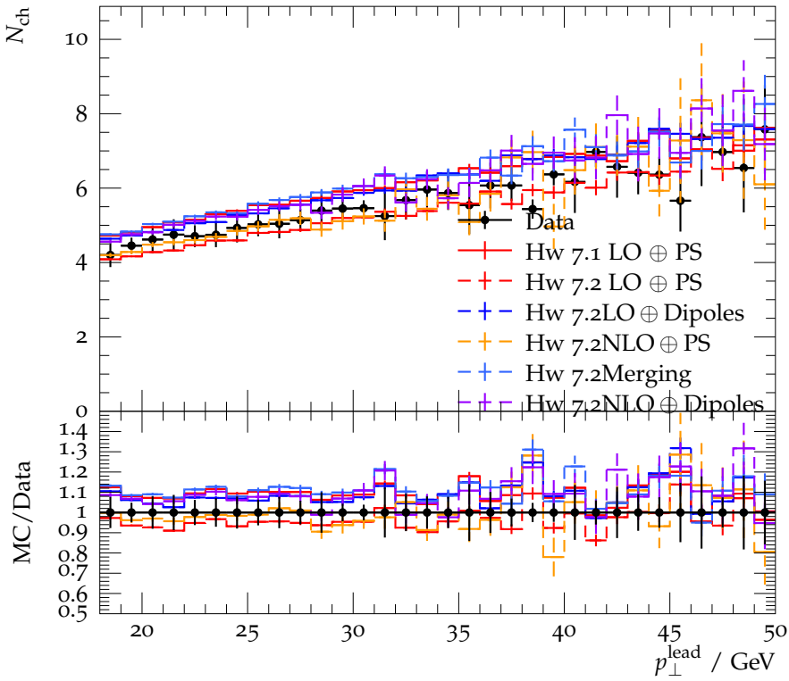
N_{\text{ch}} (away) for JET20
