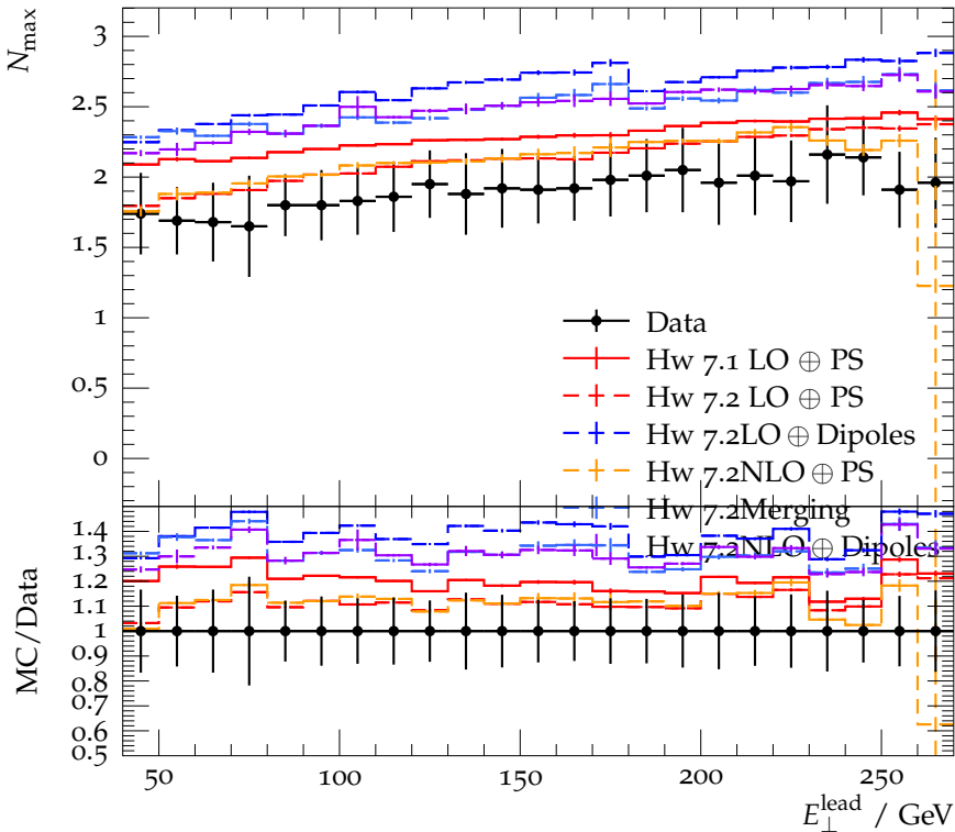
Transverse cone N_{\max} vs. E_{\perp}^{\text{lead}} at \sqrt{s} = 1800 GeV
