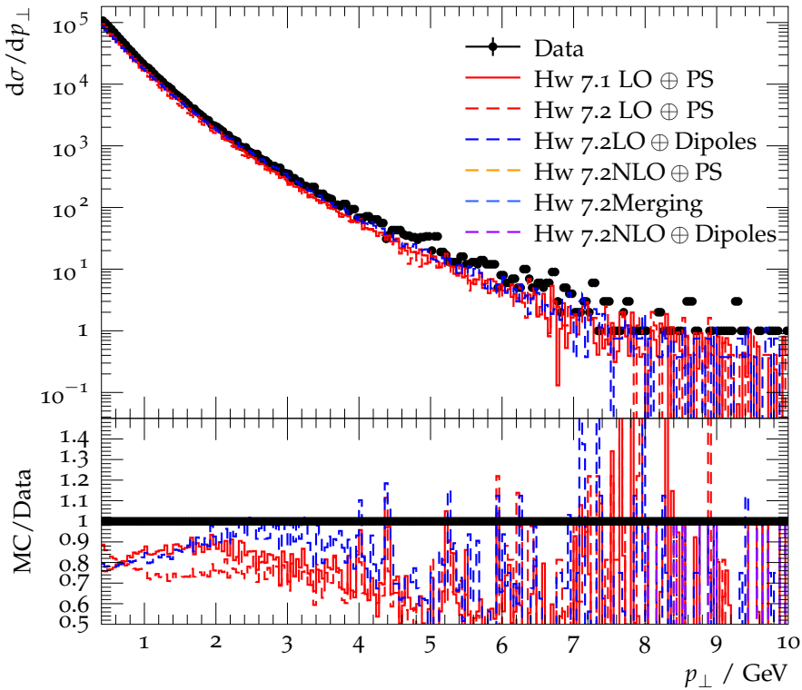
Min bias p_{\perp} distribution at \sqrt{s} = 1800 GeV
