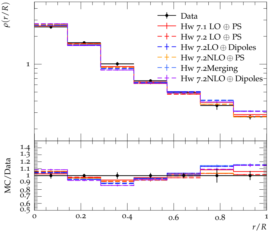
Differential jet shape \rho , 45 \text{ GeV}/c < p_{\perp}^{\text{jet}} < 55 \text{ GeV}/c
