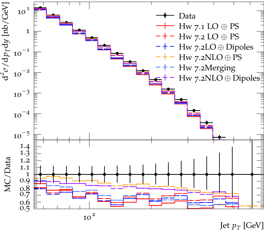
Inclusive jet cross-section vs p_T for 0.1 < |\eta| < 0.7, D = 0.7
