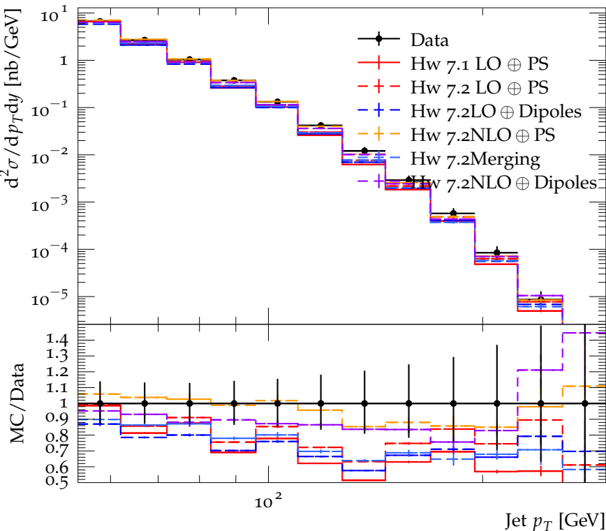
Inclusive jet cross-section vs p_T for 1.6 < |\eta| < 2.1, D = 0.7
