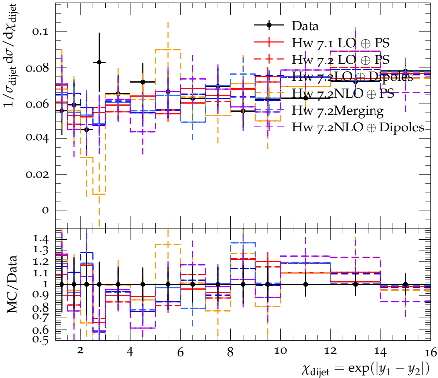
Dijet angular distribution in 0.3 < M_{jj}/\text{TeV} < 0.4
