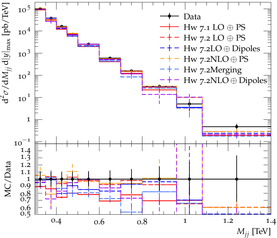
Dijet invariant mass for 1.2 < |y|_{\max} < 1.6
