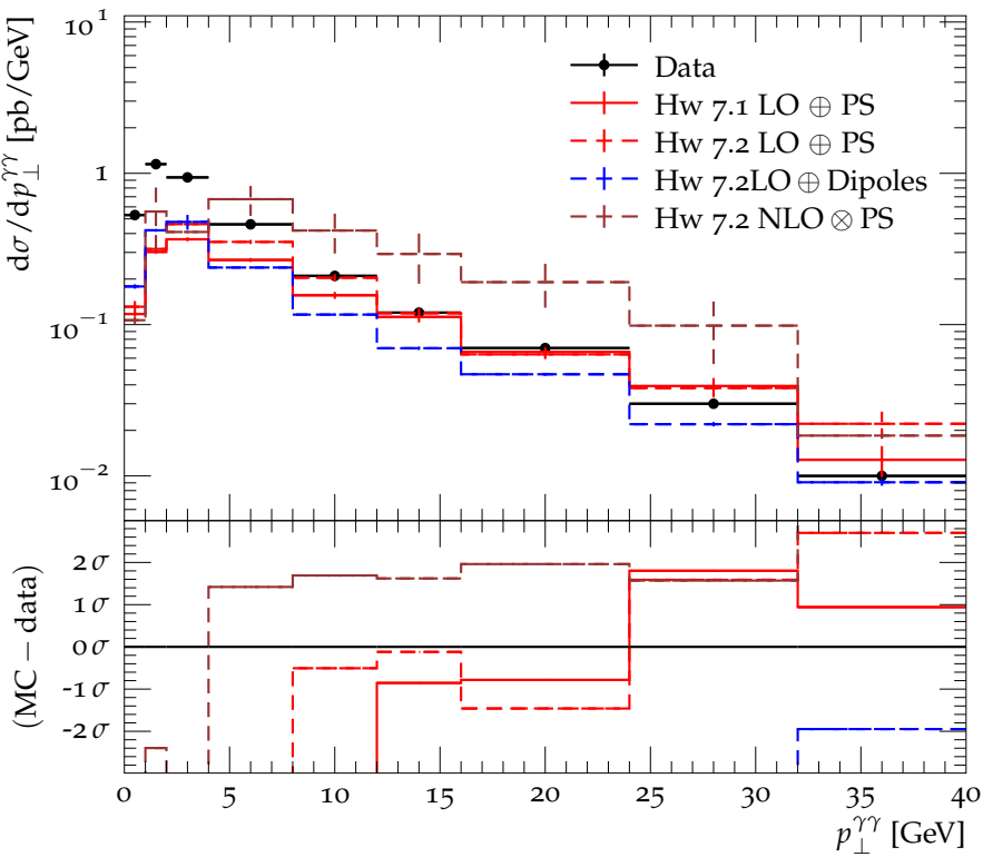
Transverse momentum of diphoton pair (compared to PYTHIA)
