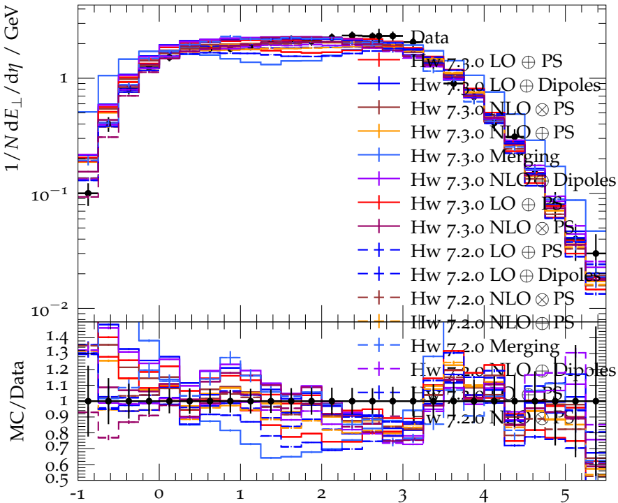
Transverse energy flow as a function of rapidity, x > 10^{-3}
