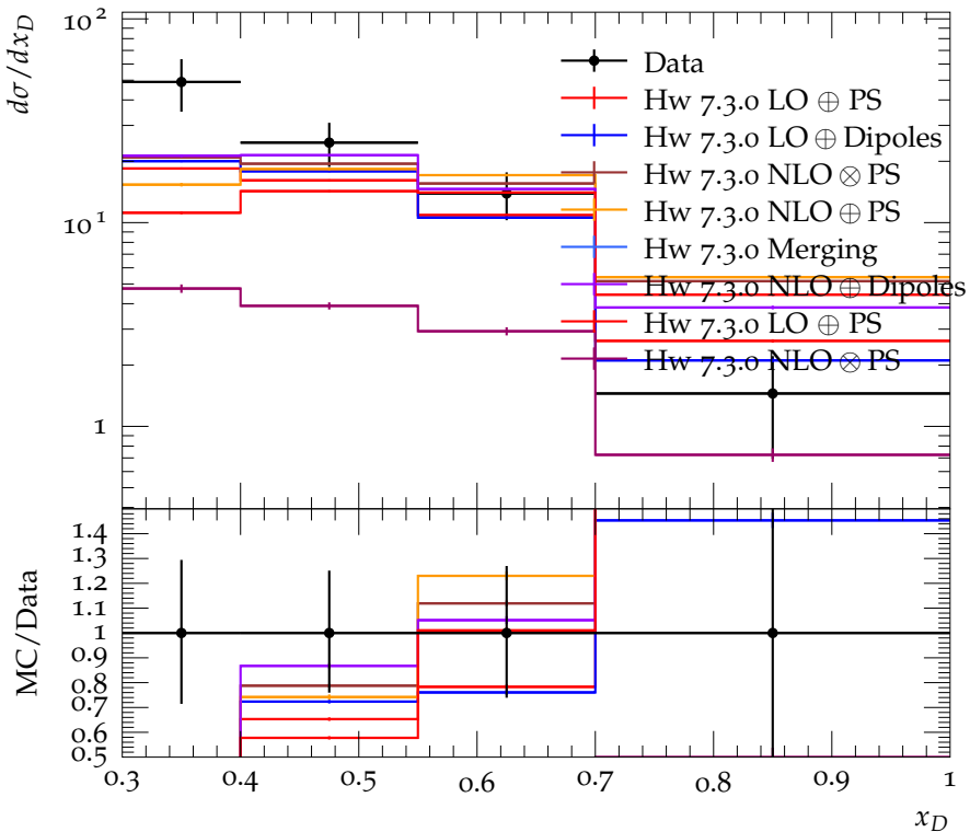
x_D Distribution for D^0
