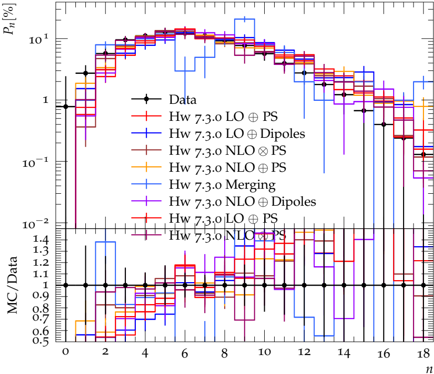
P_n vs multiplicity 1 < \eta < 4, 80 < W < 115 GeV
