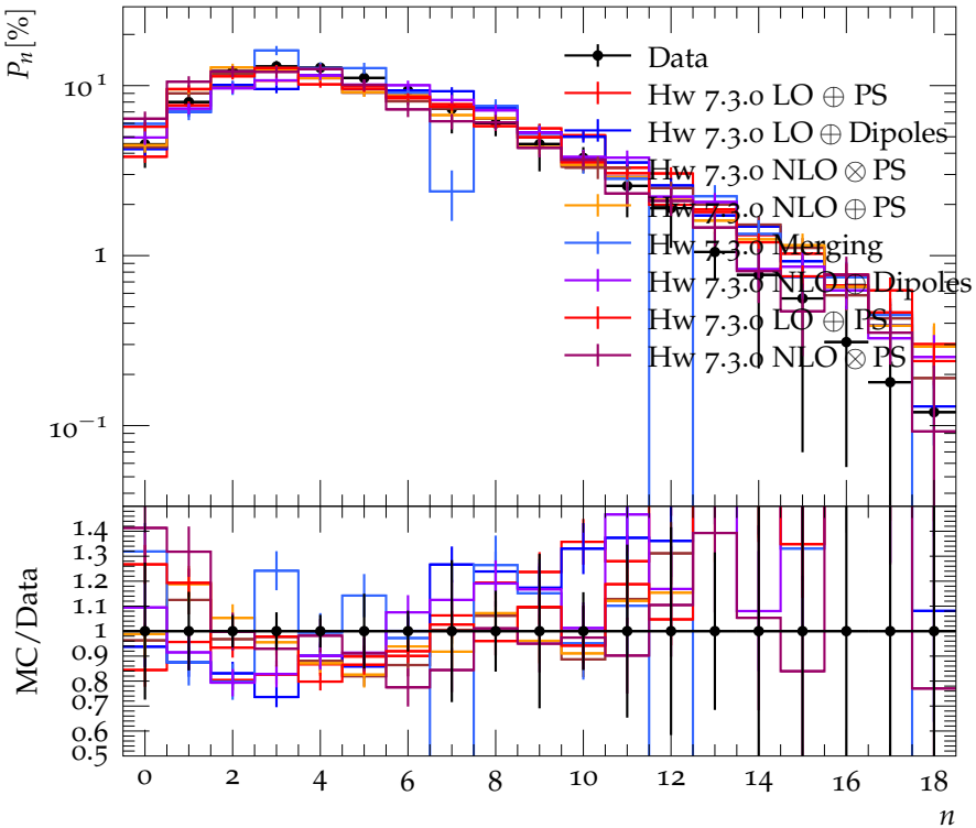
P_n vs multiplicity 1 < \eta < 3 , 115 < W < 150 GeV
