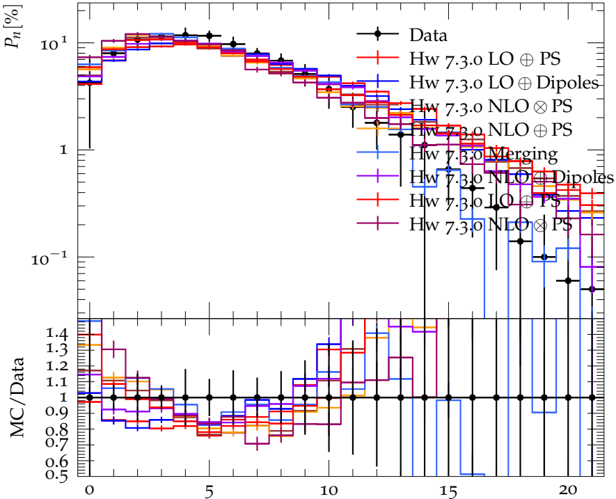
P_n vs multiplicity 1 < \eta < 3 , 185 < W < 220 GeV
